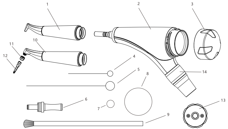
Fig. 1 AirJet 2 Structure and Accessories
